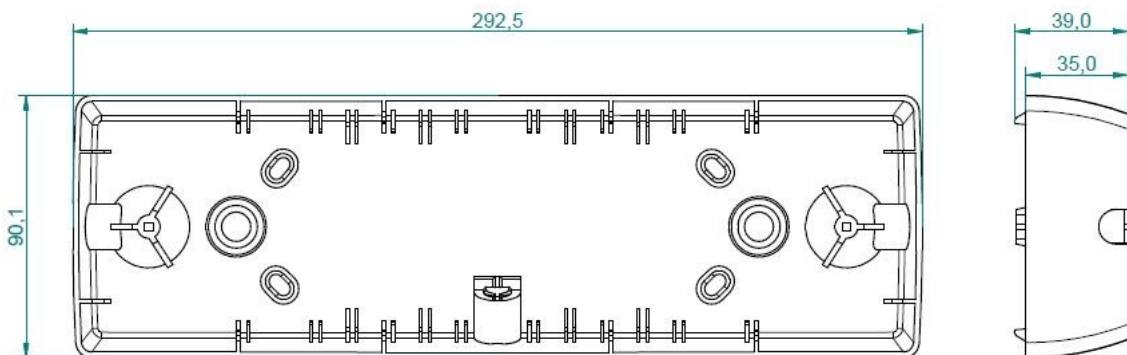
11802/6 Surface Box
